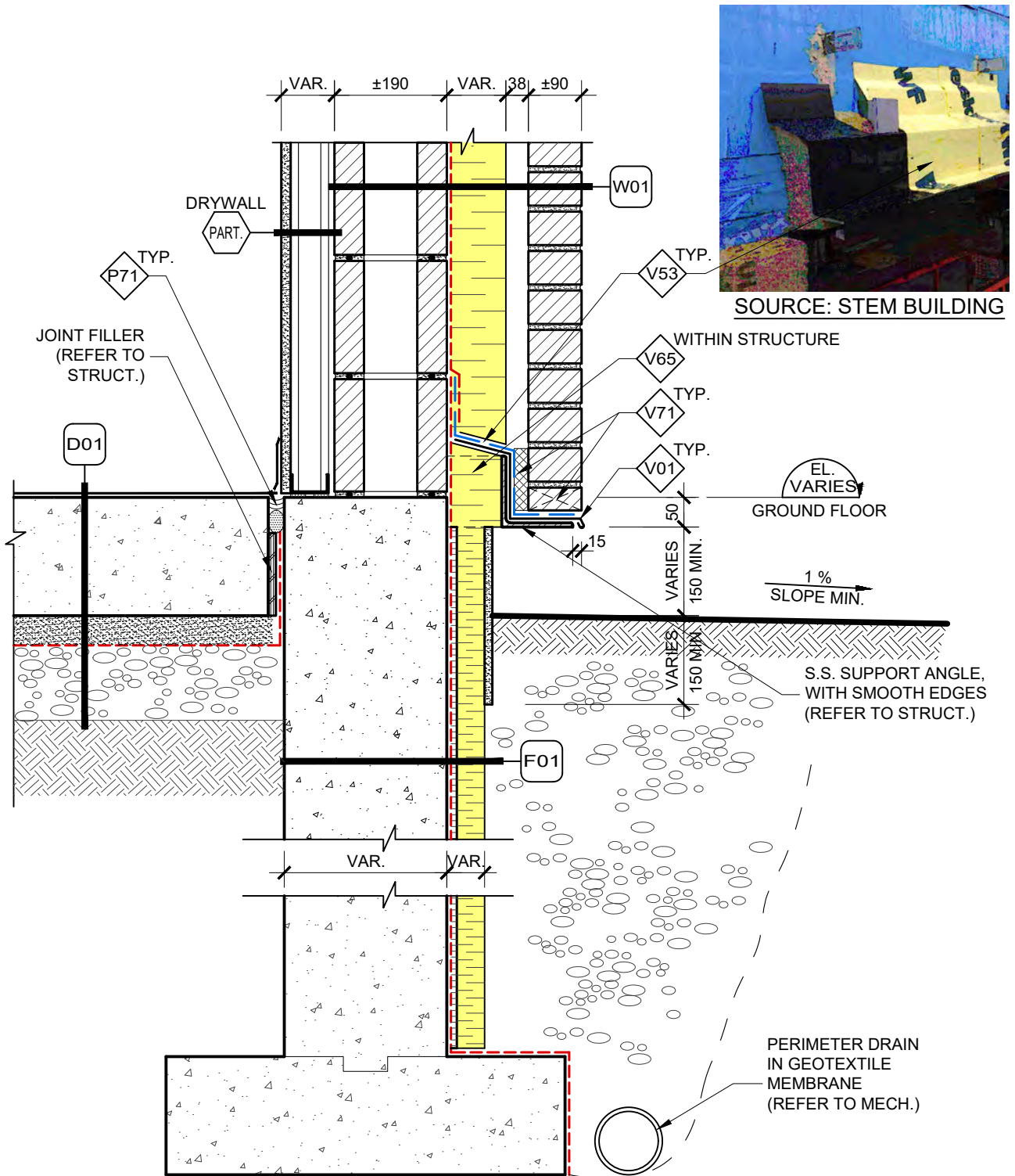
MASONRY CLADDING FOUNDATION - RECESSED EDGE SECTION DETAIL (TYPICAL)
