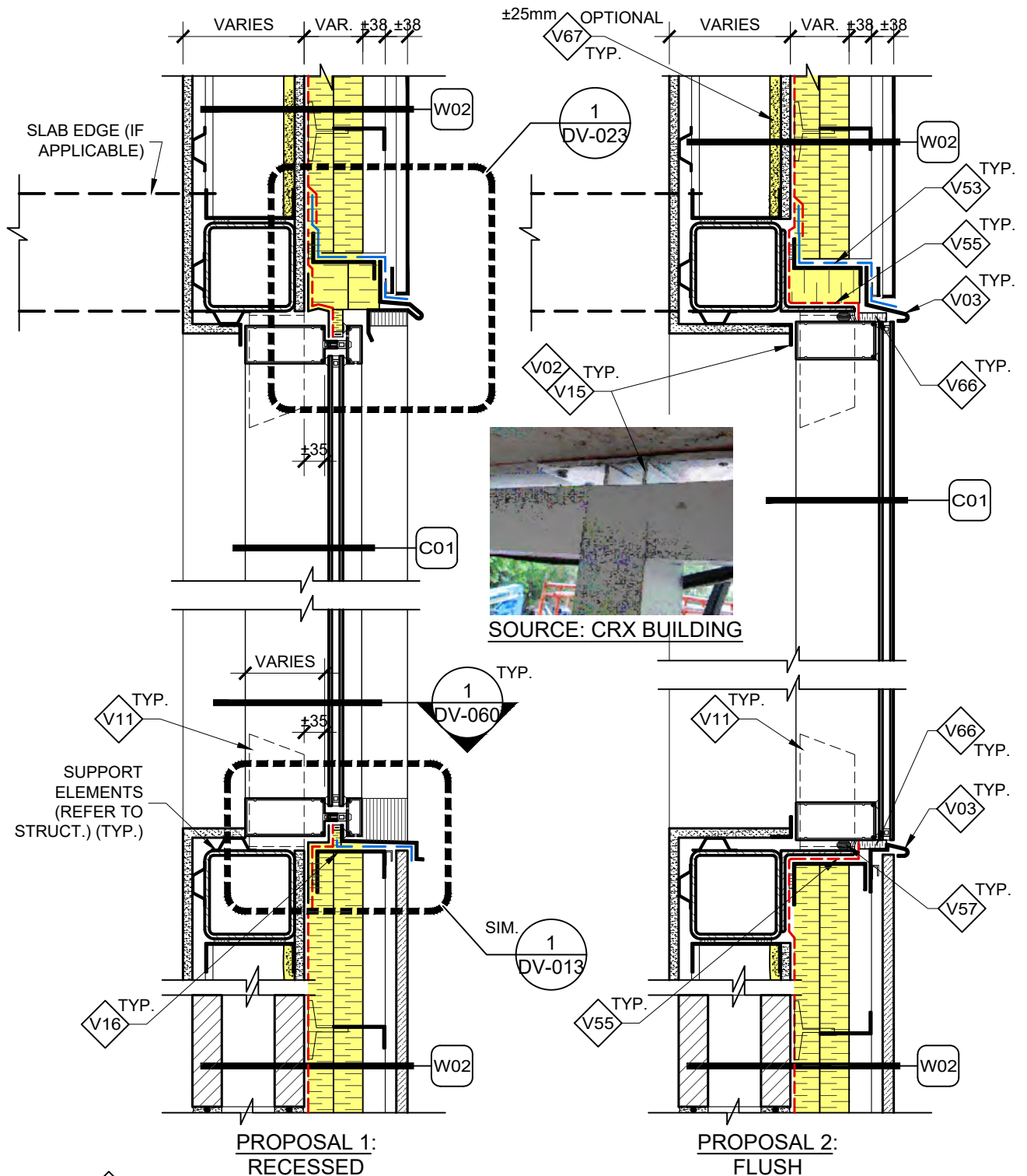
A01 1 DV-022 CURTAIN WALL HEAD AND SILL - PANEL CLADDING SECTION DETAIL (TYPICAL)
