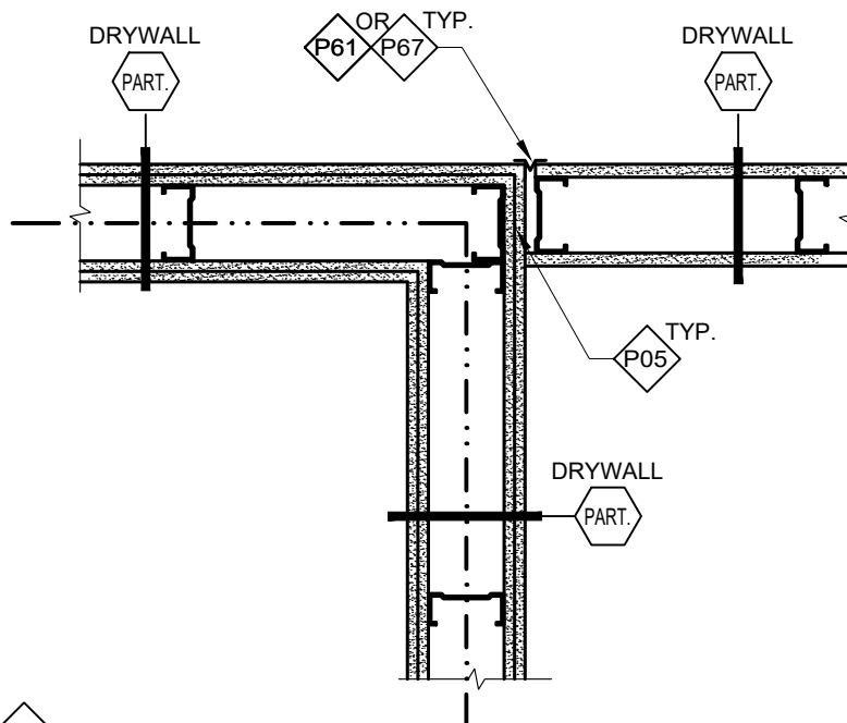
2 CONNECTION WITH FRR PARTITION DP-050 PLAN DETAIL (TYPICAL) SCALE: 1:10
