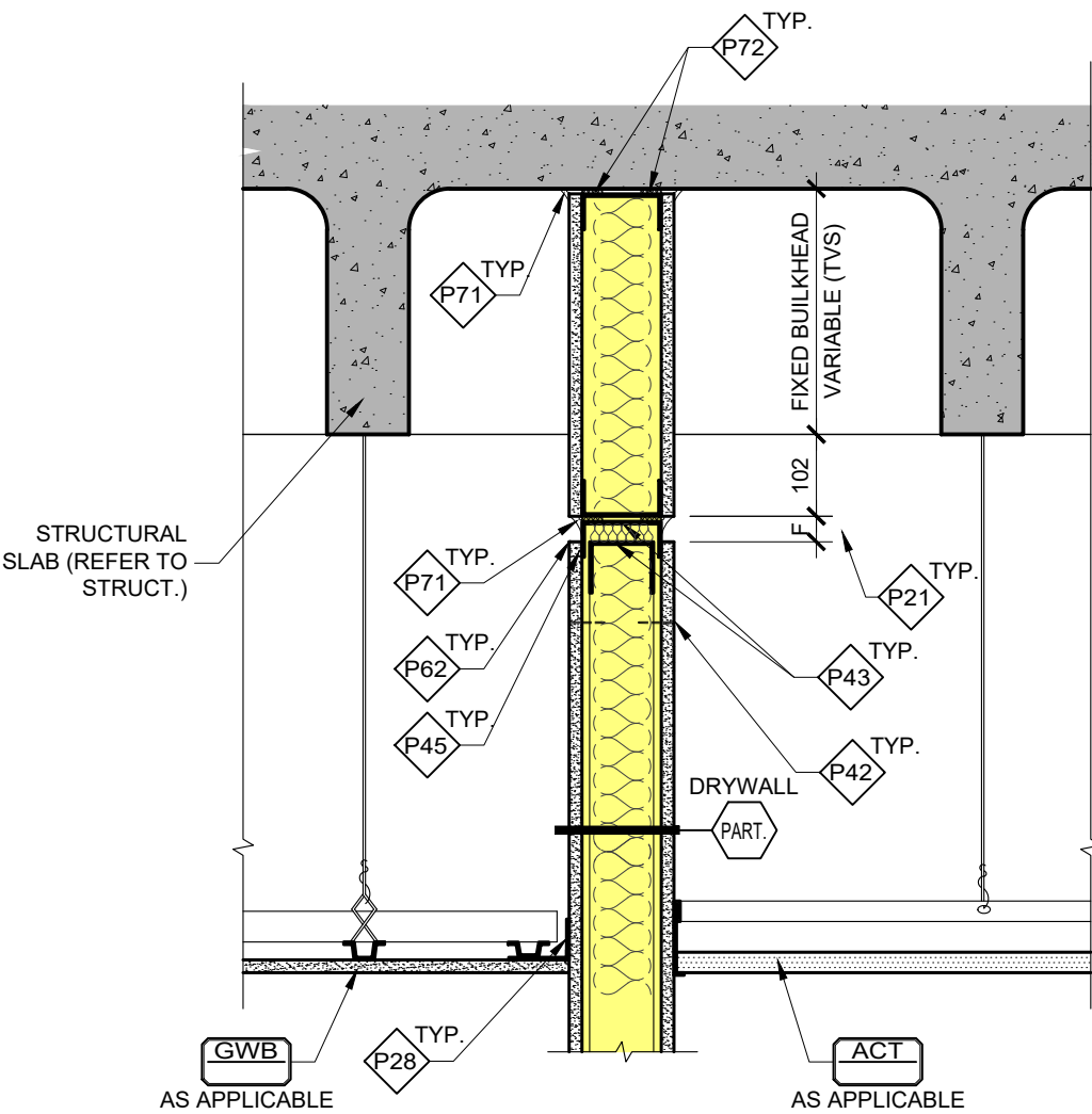
1 DP-021 A01 FULL HEIGHT PARTITION HEAD U/S SLAB - DRY WALL SECTION DETAIL (TYPICAL) SCALE: 1:10
