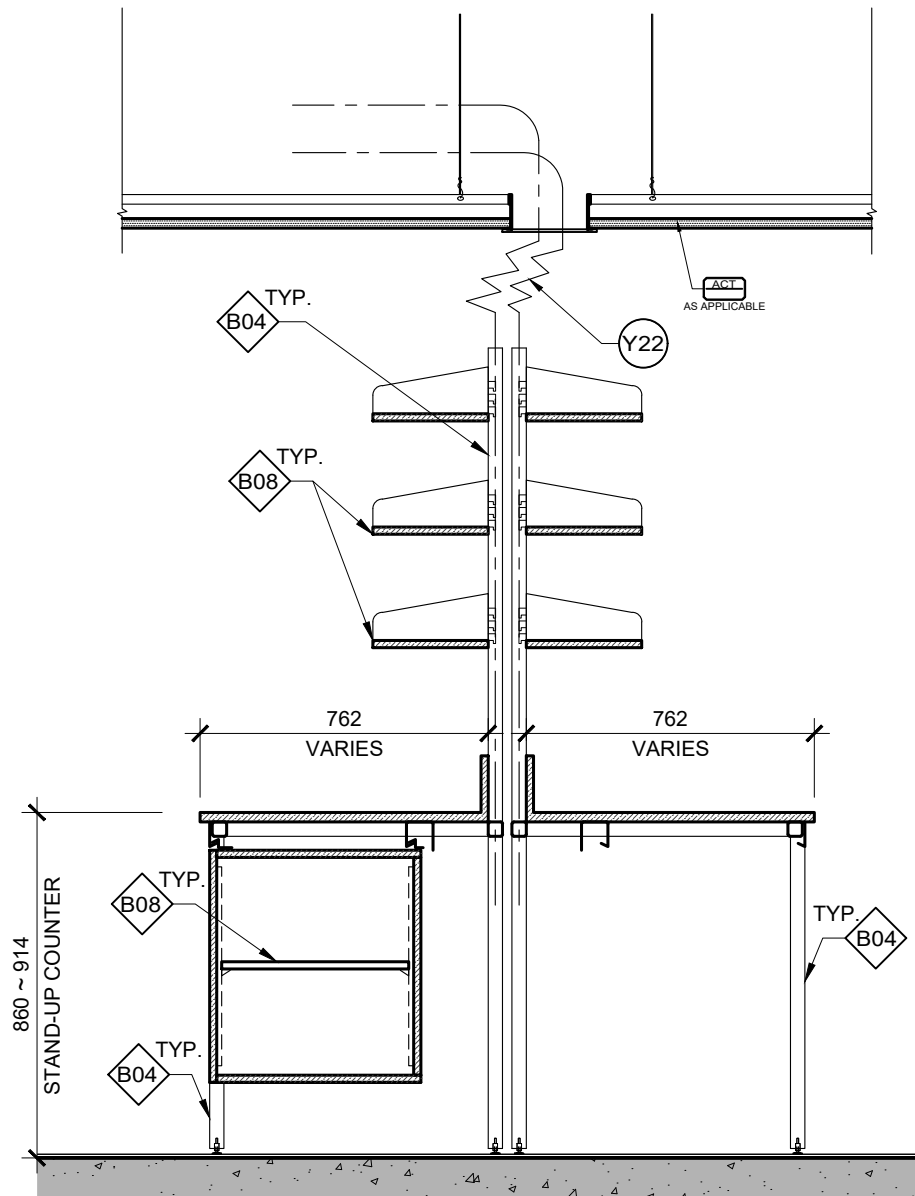
1 MOVABLE COUNTERTOP - ISLAND UNITS DB-022 SECTION (TYPICAL) SCALE: 1:20
