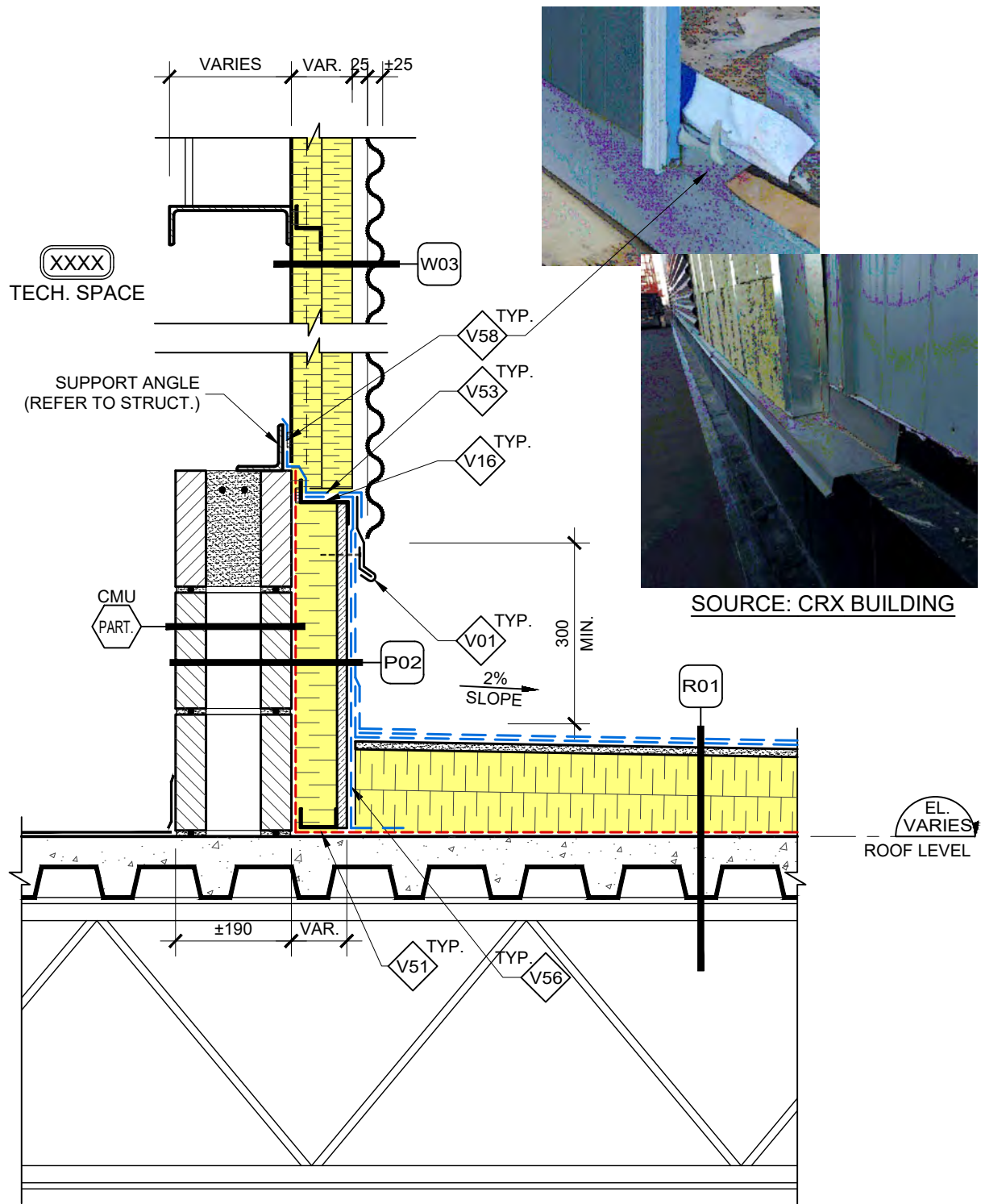
A01 1 DV-033 CORRUGATED METAL CLADDING - STUD PARAPET ROOF EXTENSION SECTION DETAIL (TYPICAL) SCALE: 1:10
