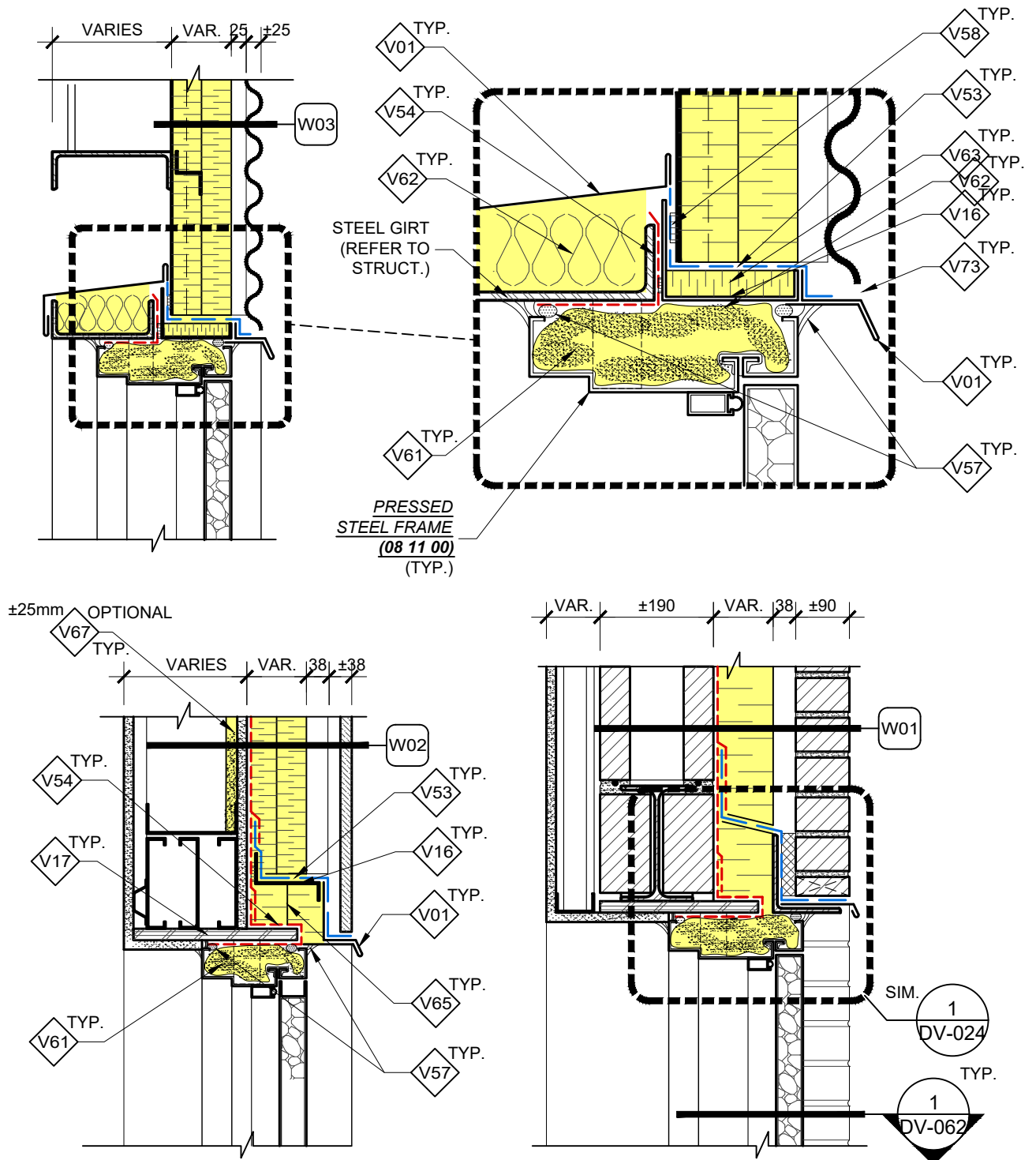
PRESSED STEEL FRAME HEADS SECTION DETAIL (TYPICAL)
