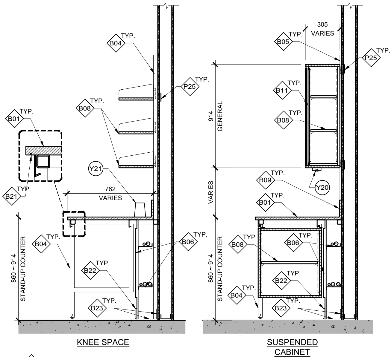
1 DB-020 FIXED COUNTERTOP - WALL UNITS SECTION (TYPICAL) SCALE: 1:20
