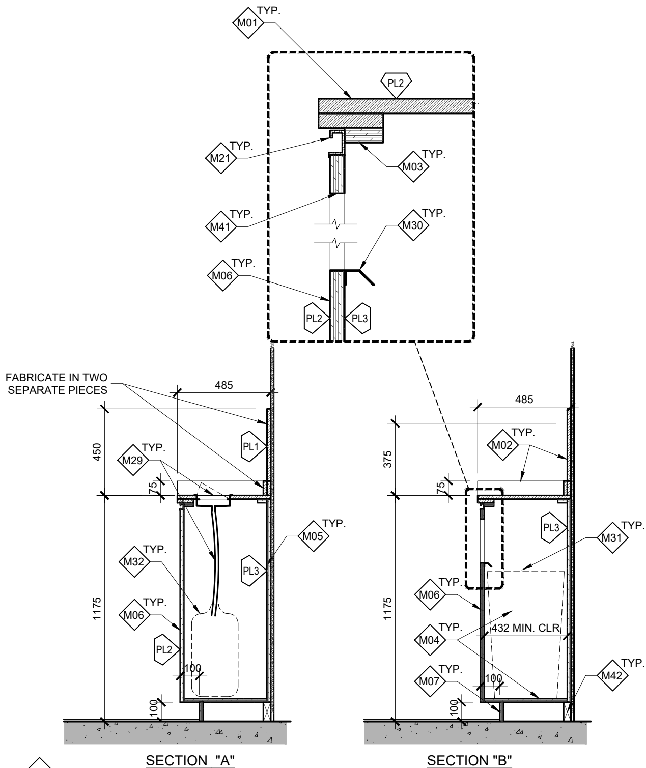
1 A01 WASTE RECYCLING STATION SECTION DETAILS (TYPICAL)
