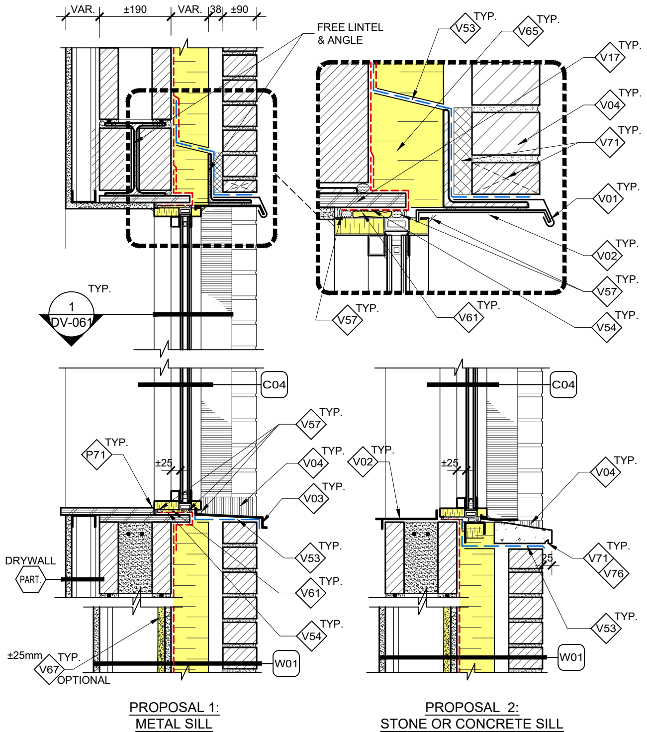
1 WINDOW UNIT HEAD AND SILL - MASONRY CLADDING SECTION DETAIL (TYPICAL)
