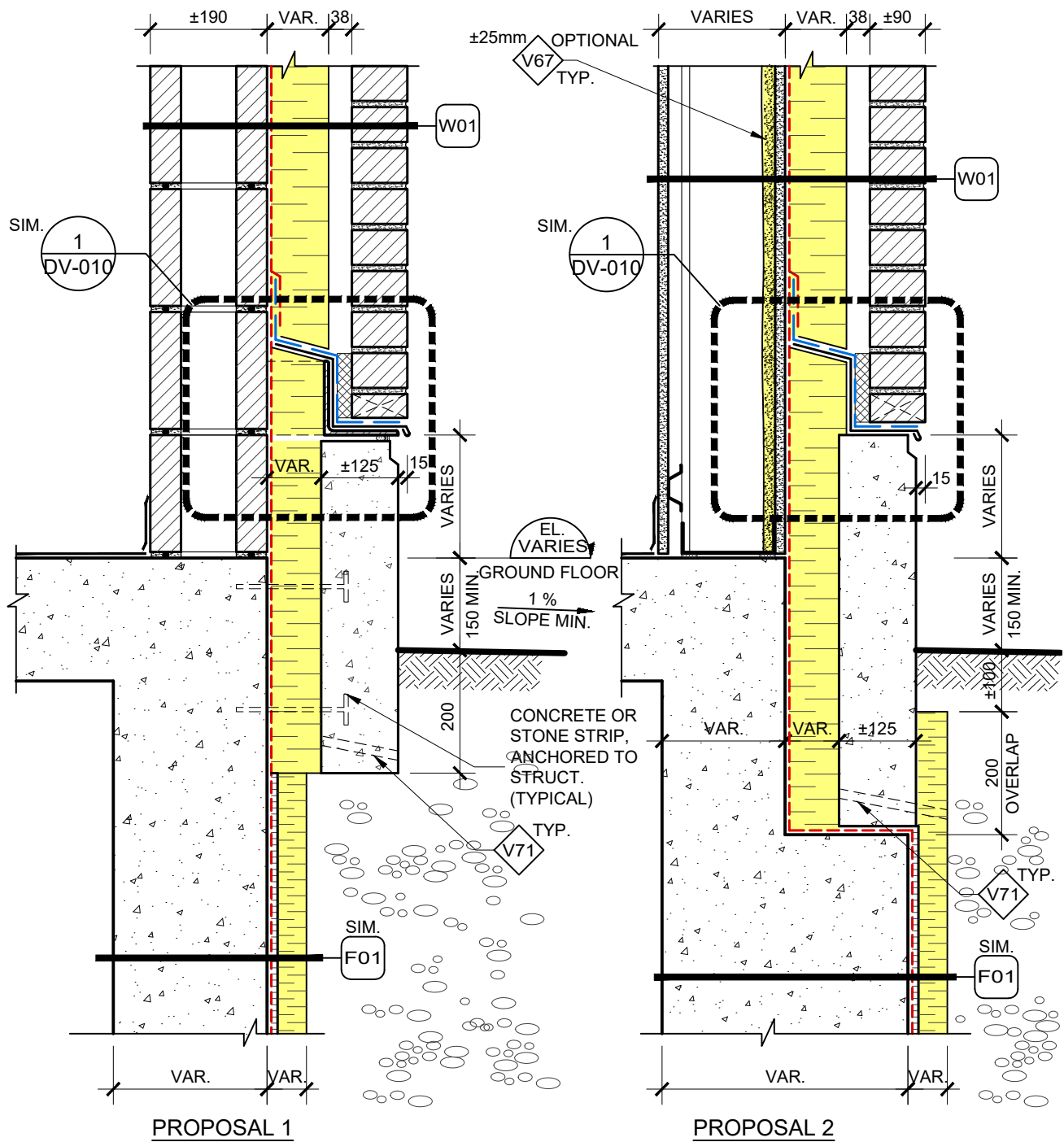
A01 1 DV-011 MASONRY CLADDING FOUNDATION - FLUSH EDGE SECTION DETAIL (TYPICAL) SCALE: 1:10
