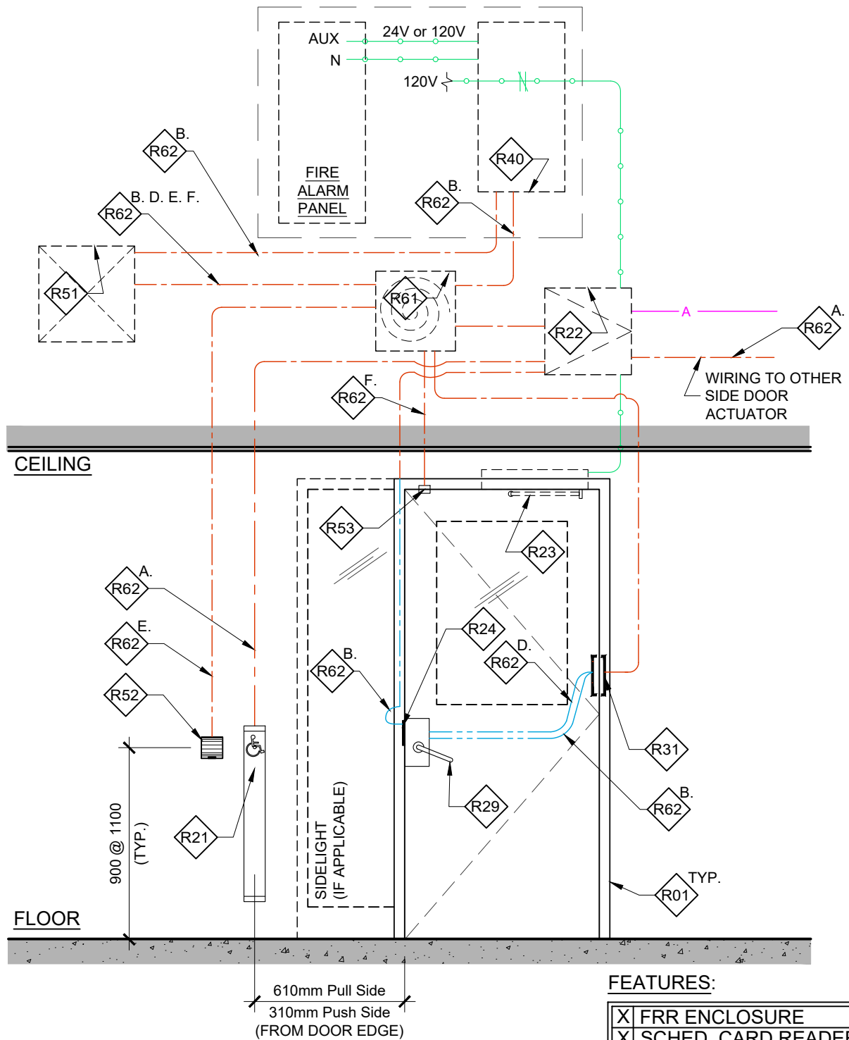
SINGLE DOOR WITH / WITHOUT SIDELIGHT
