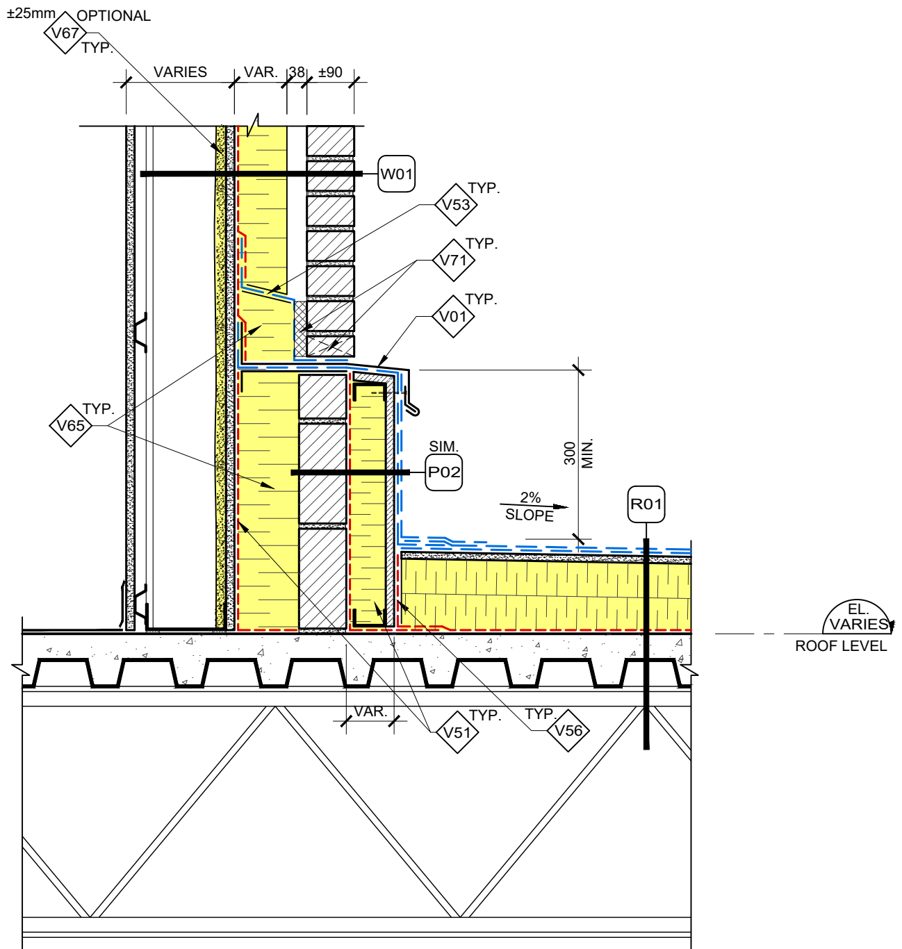
1 A01 MASONRY CLADDING - STUD PARAPET ROOF EXTENSION DV-031 SECTION DETAIL (TYPICAL) SCALE: 1:10
