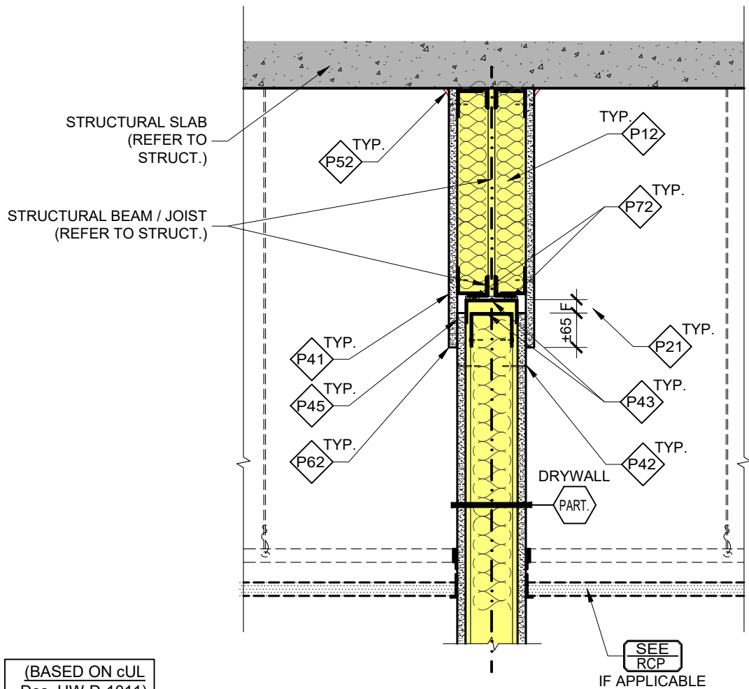
1 A01 FULL HEIGHT PARTITION HEAD U/S JOIST - DRY WALL DP-015 SECTION DETAIL (TYPICAL) SCALE: 1:10
