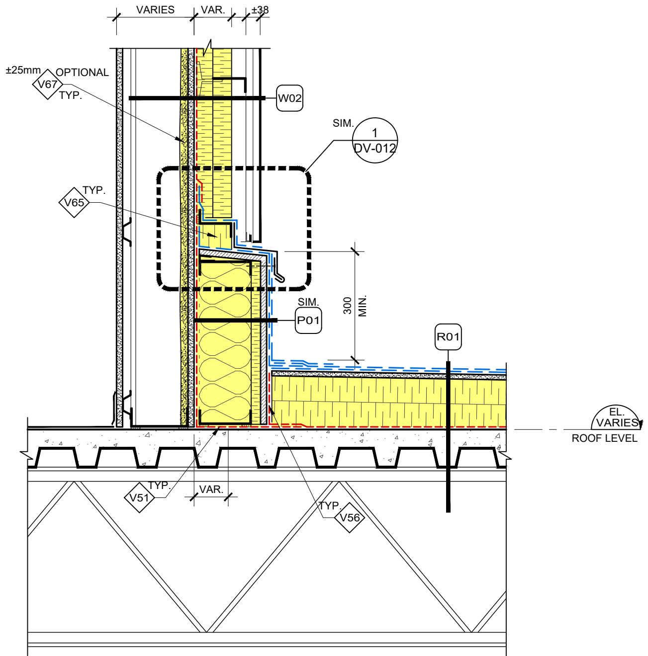
PANEL CLADDING - STUD PARAPET ROOF EXTENSION SECTION DETAIL (TYPICAL)
