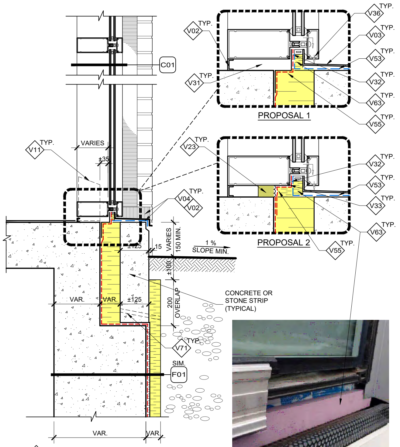
1 CURTAIN WALL BASE DV-013 SECTION DETAIL (TYPICAL)
