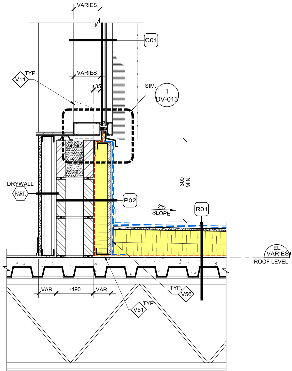
CURTAIN WALL - PARAPET ROOF EXTENSION SECTION DETAIL (TYPICAL)
