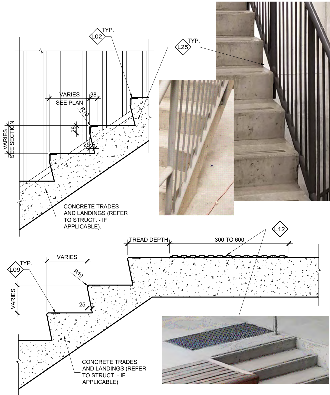
NON-INDUSTRIAL CONCRETE RISERS & HANDRAIL / BALUSTRADE SECTION DETAIL (TYPICAL)
