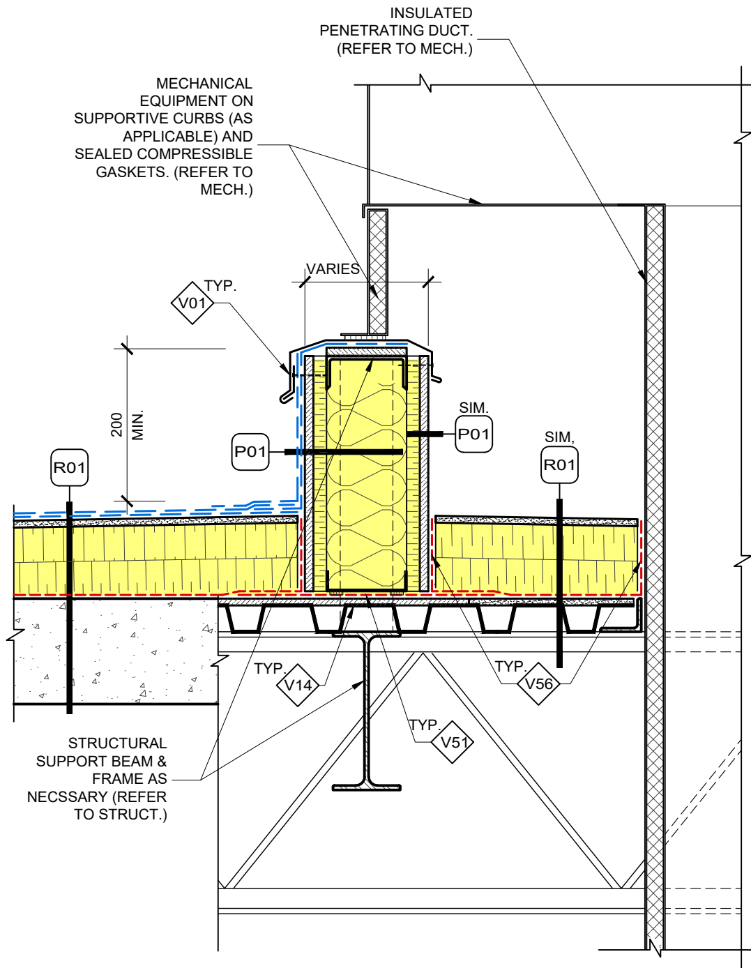
1 EQUIPMENT SUPPORT & PENETRATIONS DV-051 SECTION DETAIL (TYPICAL)
