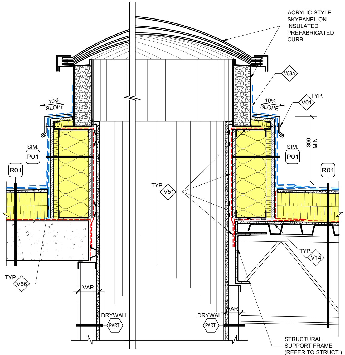
1 PREFABRICATED SKIPANELS DV-055 SECTION DETAIL (TYPICAL)
