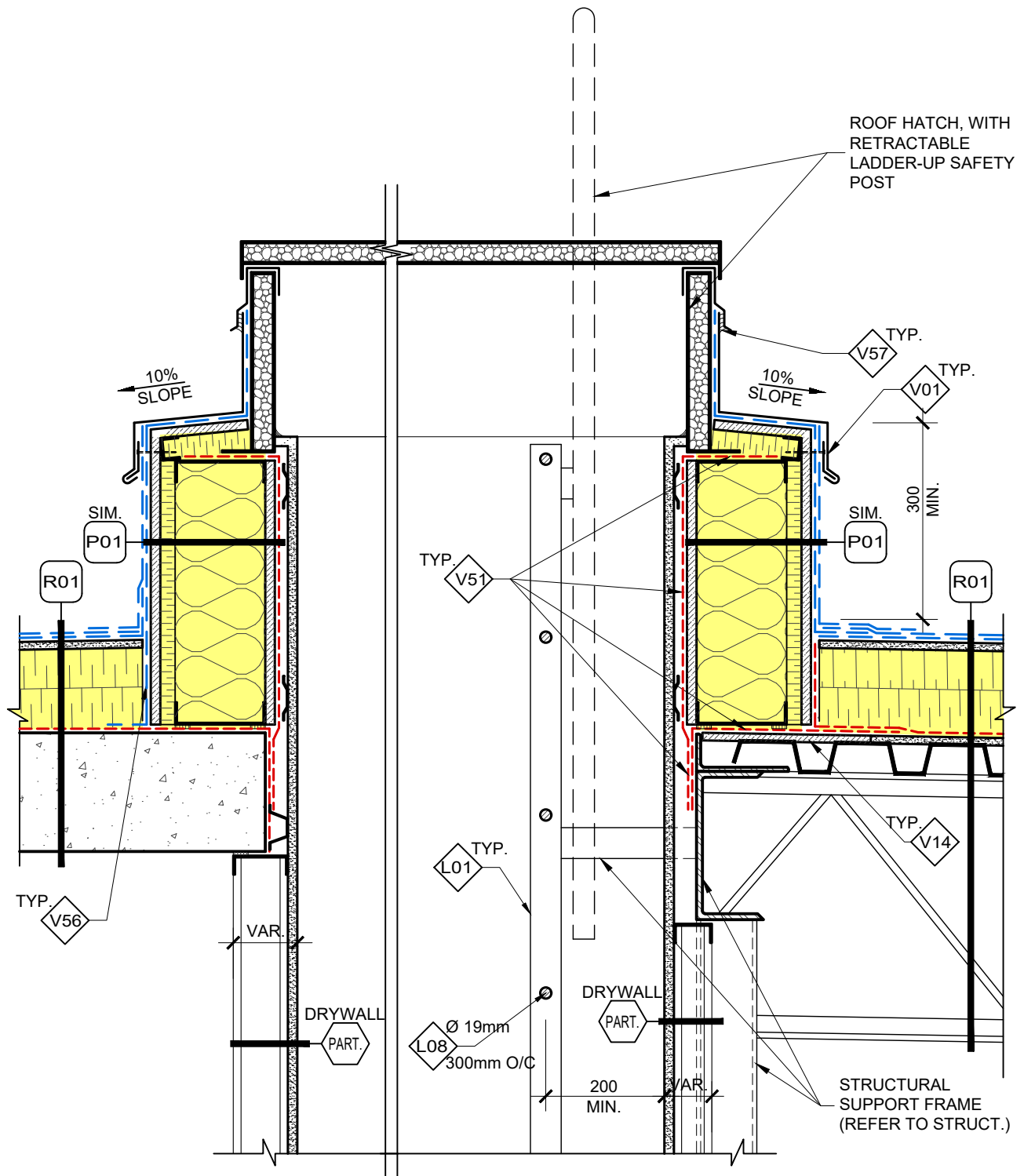
A01 1 ROOF HATCH DV-056 SECTION DETAIL (TYPICAL)
