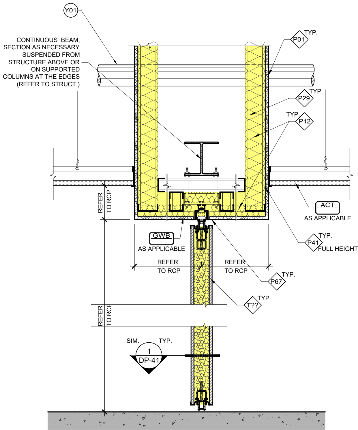
1 DP-040 MOVABLE PARTITION SECTION DETAIL (TYPICAL) SCALE: 1:10
