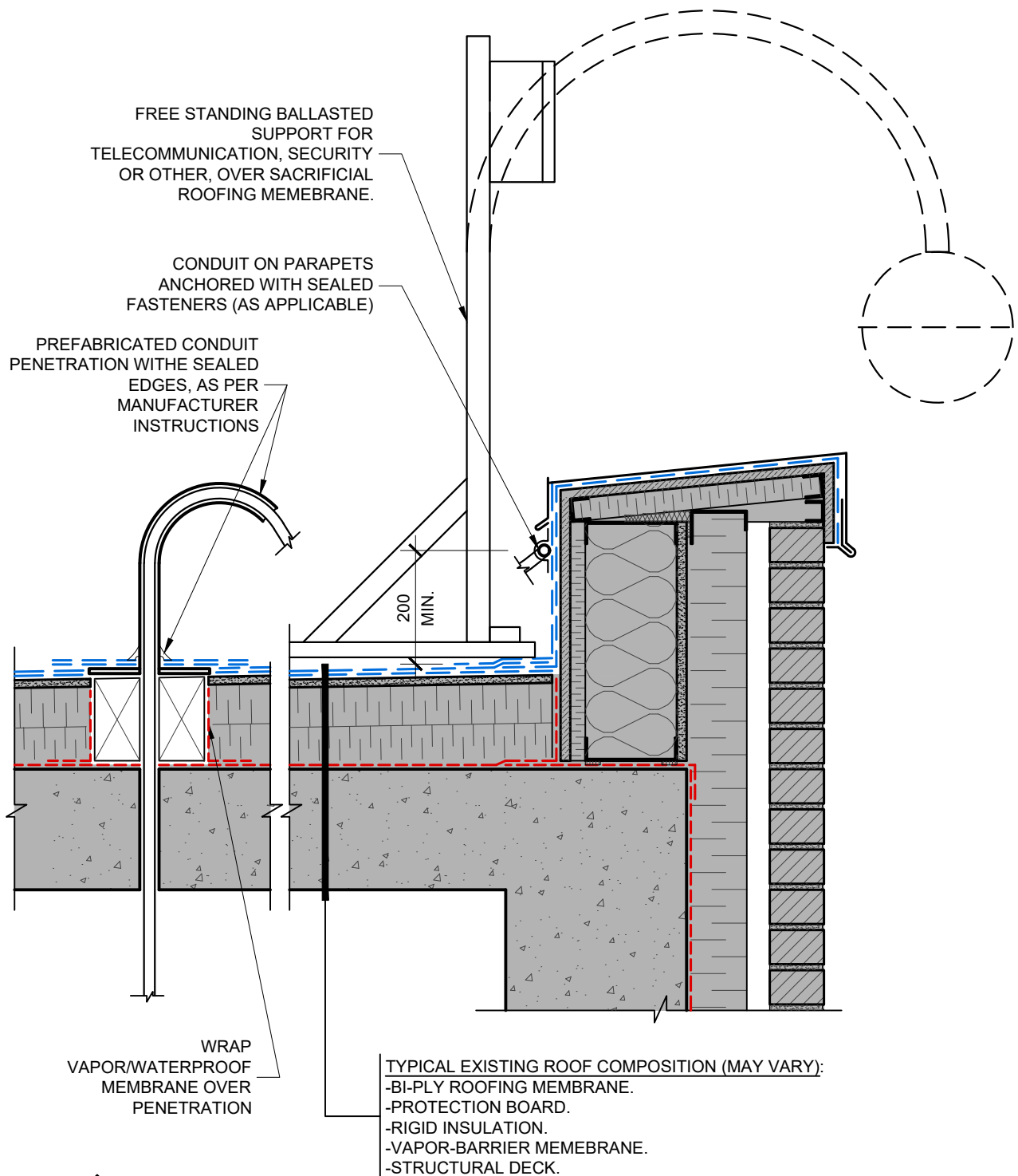
CONDUIT PENETRATION SECTION DETAIL (TYPICAL)
