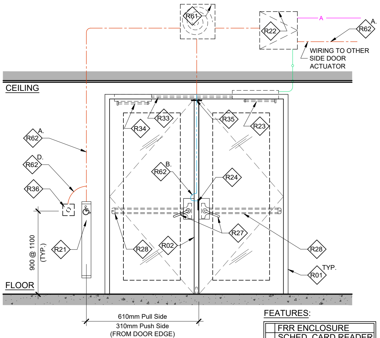
1 DOUBLE DOOR / TWO ACTIVE LEAVES DR-055
