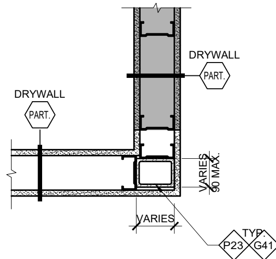
1 FREE STANDING PARTITION DP-050 PLAN DETAIL (TYPICAL) SCALE: 1:10
