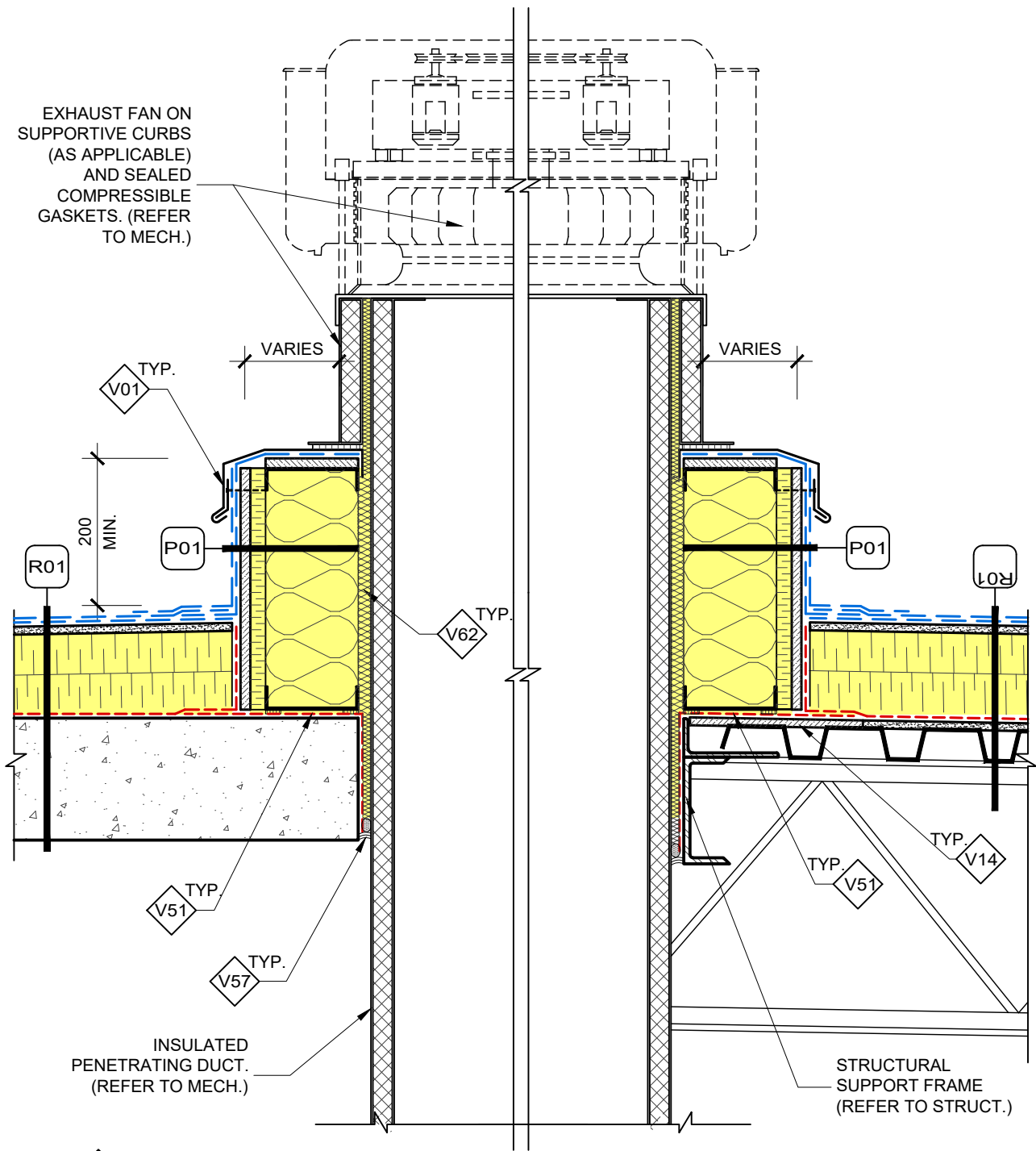
1 A01 EXHAUST FAN, AIR INTAKE OR GOOSENECK SECTION DETAIL (TYPICAL) SCALE: 1:10
