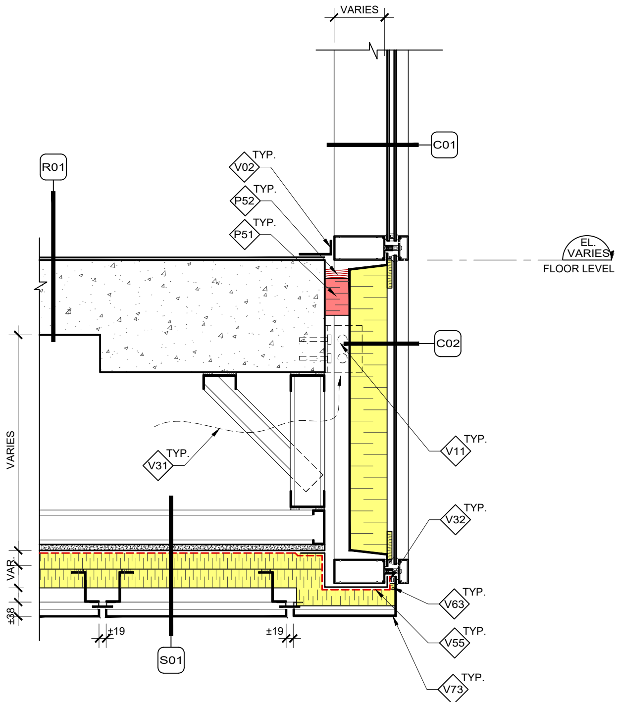
1 CURTAIN WALL - HEATED SOFFIT CONNECTION DV-047 SECTION DETAIL (TYPICAL) SCALE: 1:10
