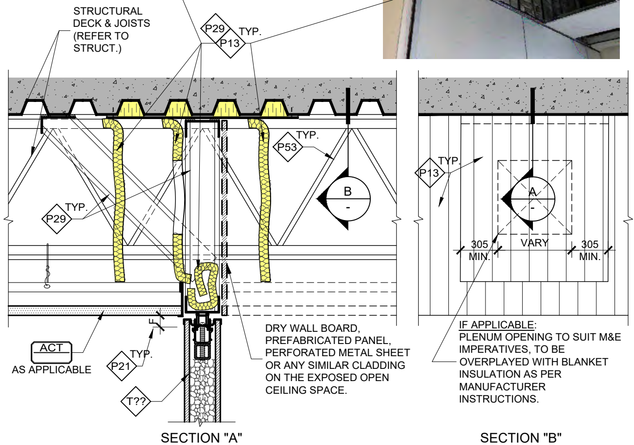
1 NON FULL-HEIGHT PARTITION HEAD - DEMOUNTABLE OR FIXED DP-023 SECTION DETAIL (TYPICAL)
