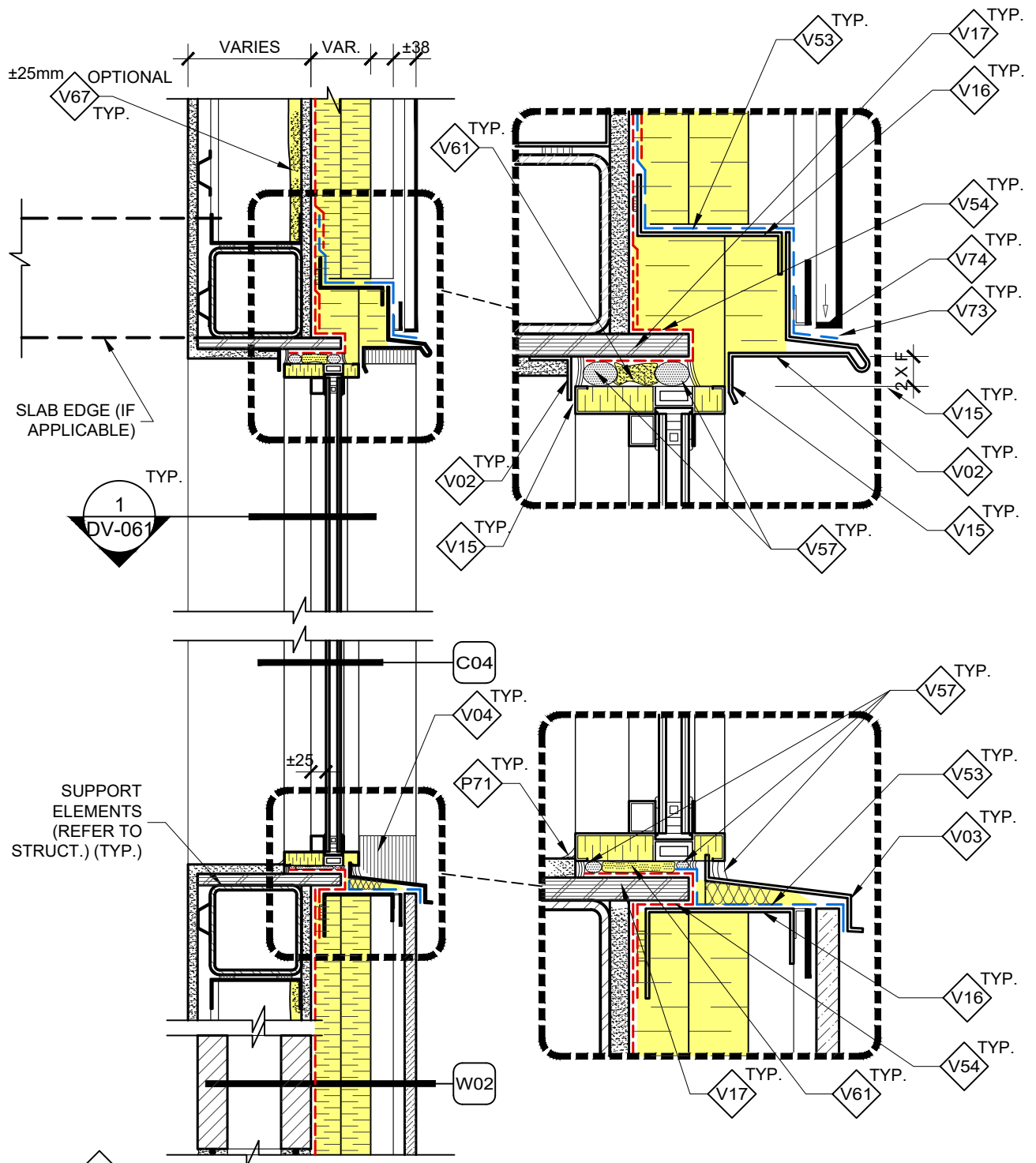
1 A01 1 DV-025 WINDOW CONTINUOUS TRIP HEAD AND SILL - PANEL CLADDING SECTION DETAIL (TYPICAL)
