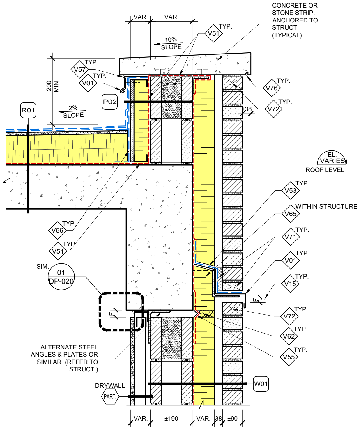
A01 1 MASONRY CLADDING - CMU PARAPET DV-040 SECTION DETAIL (TYPICAL) SCALE: 1:10
