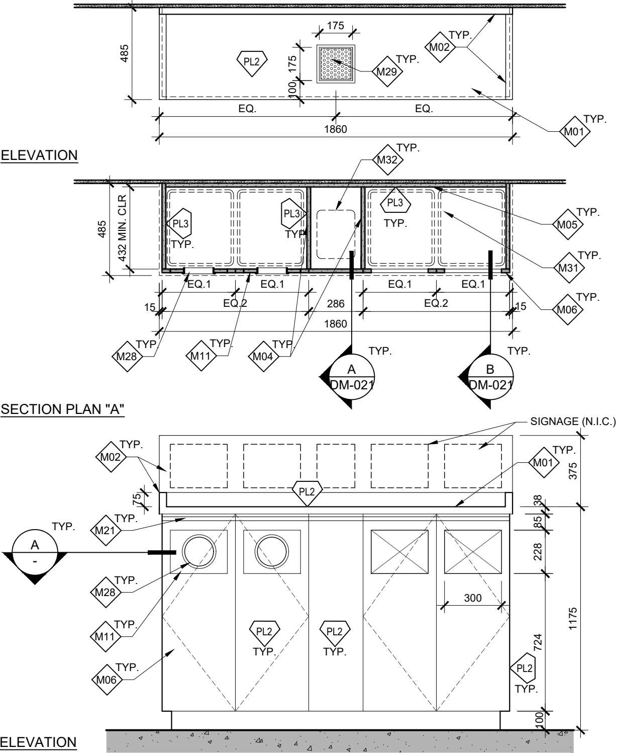
1 A01 WASTE RECYCLING STATION OVERALL VIEW (TYPICAL) SCALE: 1:20
