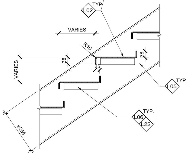
INDUSTRIAL OPEN RISERS & HANDRAIL / BALUSTRADE SECTION DETAIL (TYPICAL)
