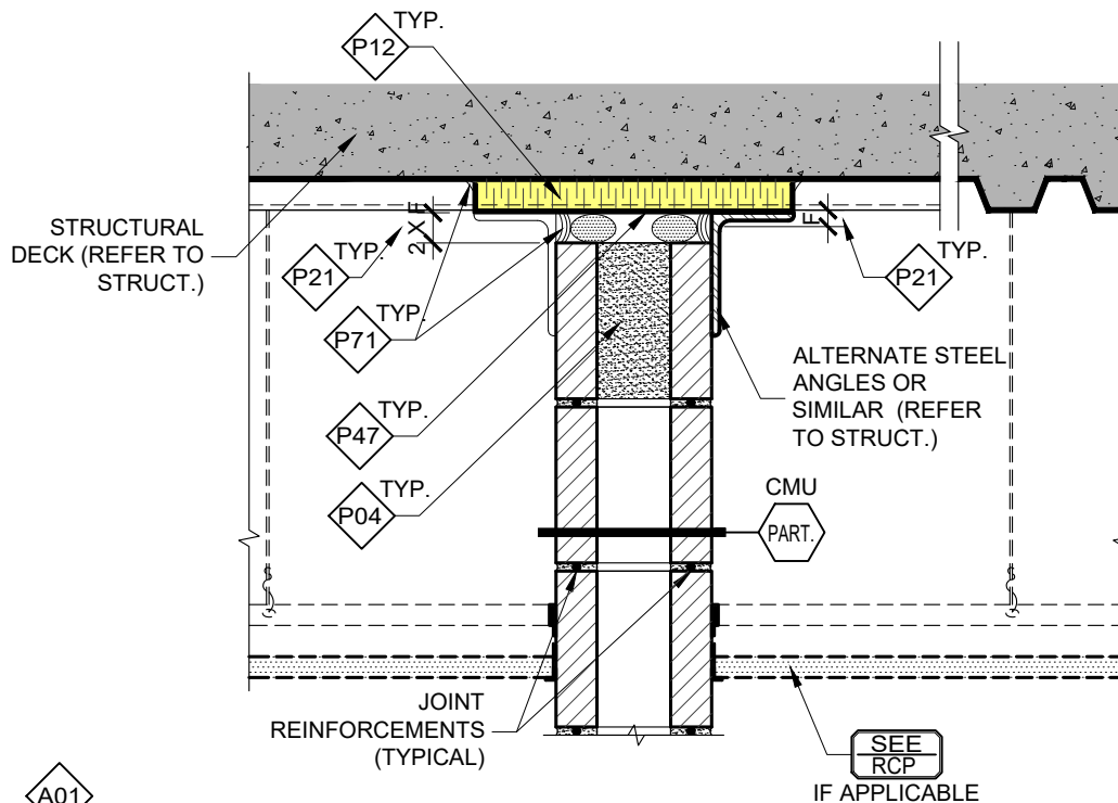
A01 1 DP-020 FULL HEIGHT PARTITION HEAD U/S SLAB - DRY WALL SECTION DETAIL (TYPICAL) SCALE: 1:10
